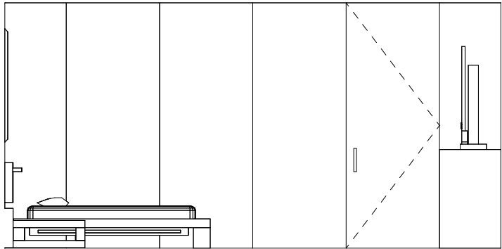
NORTH STANDARD ROOM 1/4" = 1'-0"
