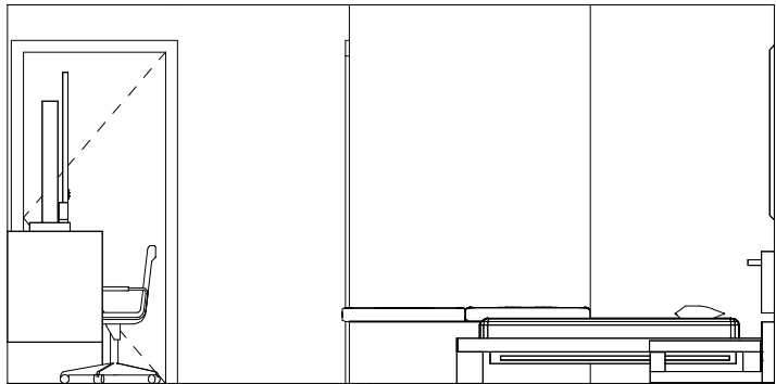
SOUTH STANDARD ROOM 1/4" = 1'-0"
