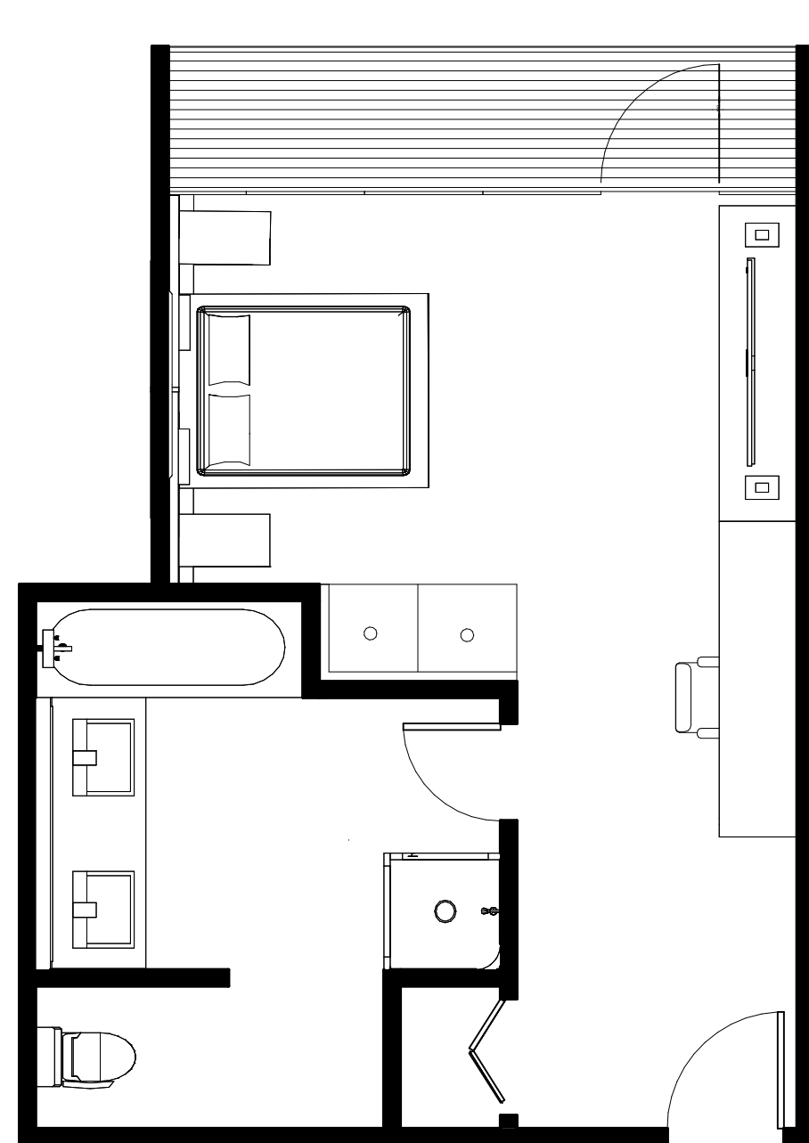
STANDARD ROOM FLOOR PLAN 1/4" = 1'-0"
