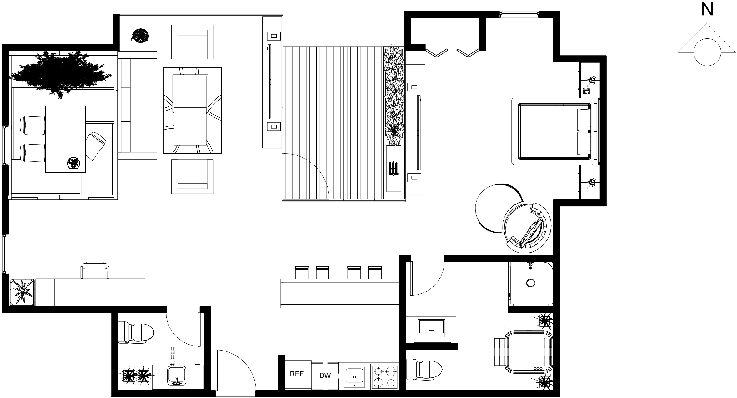
1 SUITE ROOM FLOOR PLAN 1/4" = 1'-0"
