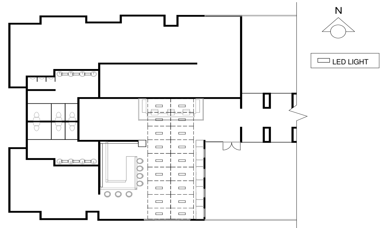
LOBBY RCP
